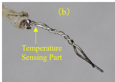
Figure 3. Temperature Sensing Part of Thermocouples
